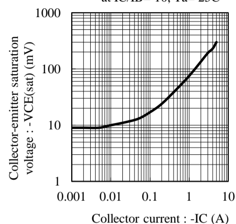
Fig.3 V_{CE(sat)} - I_C at I_C/I_B = 10, T_a = 25^\circ C
