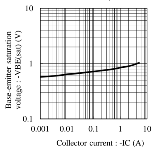
Fig.6 V_{BE(sat)} - I_C at I_C/I_B = 20, T_a = 25^\circ C
