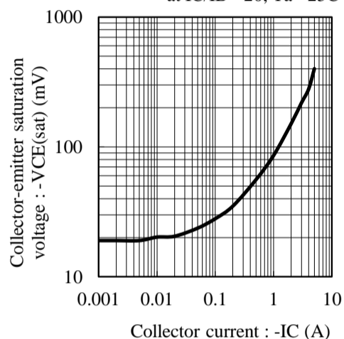
Fig.4 V_{CE(sat)} - I_C at I_C/I_B = 20, T_a = 25^\circ C
