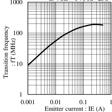
Fig.7 f_T - I_E at V_{CE} = -5V, T_a = 25^\circ C
