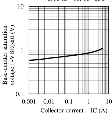
Fig.5 V_{BE(sat)} - I_C at I_C/I_B = 10, T_a = 25^\circ C
