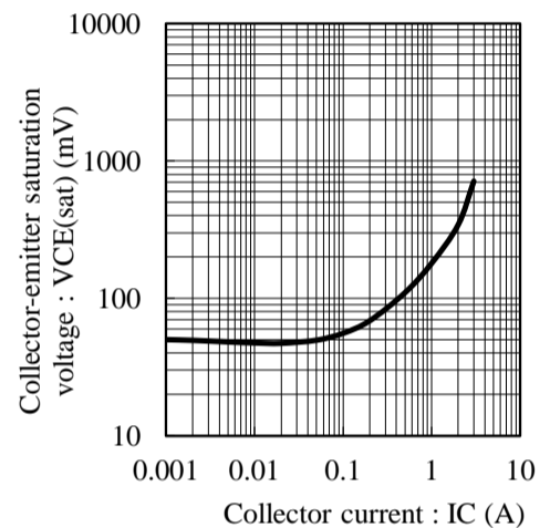
Fig.6 V_{CE(sat)} - I_C at I_C/I_B = 100, T_a = 25C
