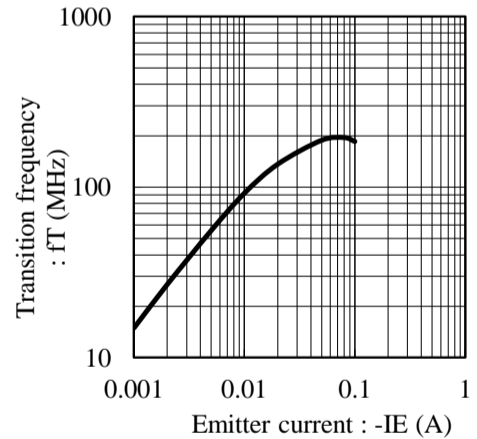
Fig.9 f_T - I_E at V_{CE} = 10V, T_a = 25C
