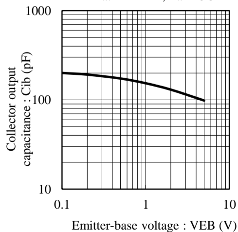
Fig.11 C_{ib} - V_{EB} at f = 1MHz, T_a = 25C
