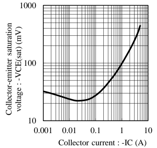
Fig.3 VCE(sat) - IC at IC/IB= 5, Ta= 25C
