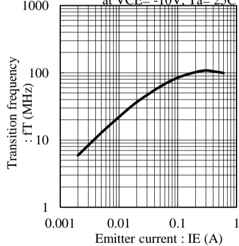
Fig.7 fT - IE at VCE= -10V, Ta= 25C
