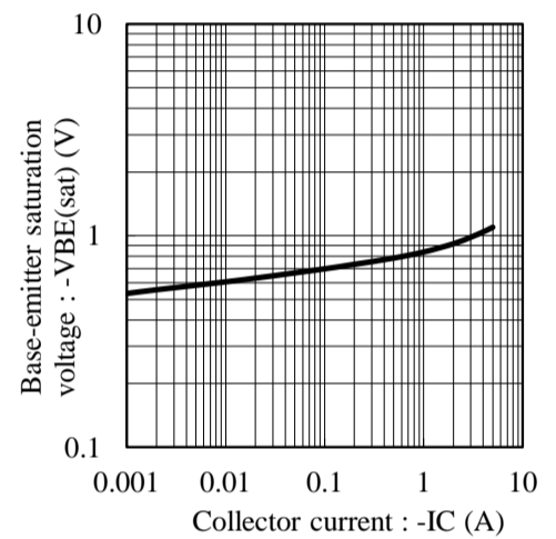
Fig.6 VBE(sat) - IC at IC/IB= 10, Ta= 25C
