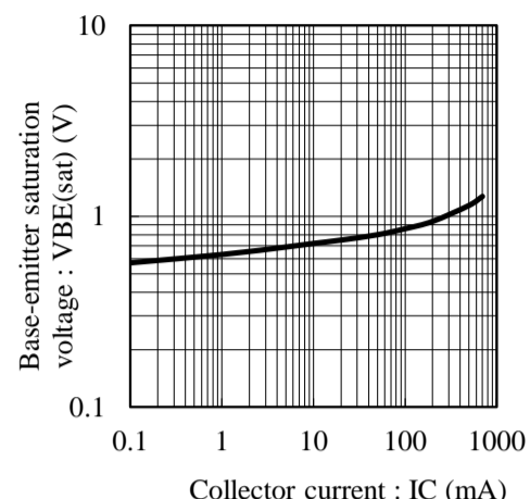
Fig.3 VBE(sat) - IC at IC/IB= 10, Ta= 25C
