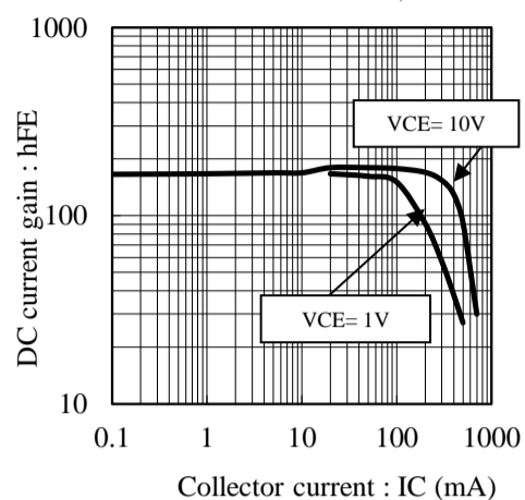
Fig.1 hFE - IC at VCE= 10V/ 1V, Ta= 25C
