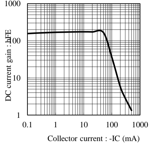
Fig.3 h_{FE} - I_C at V_{CE} = -10V, T_a = 25C
