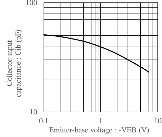
Fig.6 Cib - VEB at f= 1MHz, Ta= 25C
