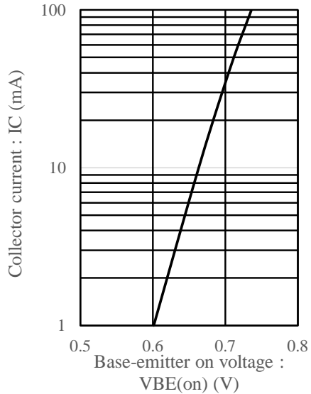
Fig.1 VBE(on) - IC at VCE= 3V, Ta= 25C
