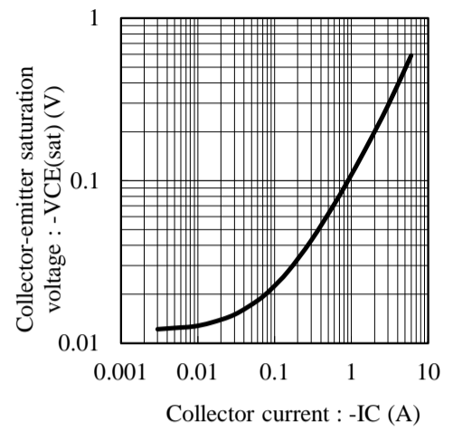
Fig.3 V_{CE(sat)} - I_C at I_C/I_B = 60, T_a = 25C
