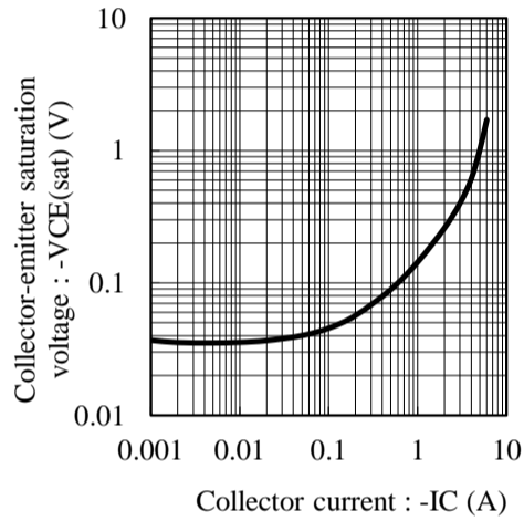
Fig.4 V_{CE(sat)} - I_C at I_C/I_B = 200, T_a = 25C
