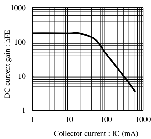
Fig.2 hFE - IC at VCE= 5V, Ta= 25C
