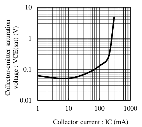
Fig.3 VCE(sat) - IC at IC/IB= 10, Ta= 25C
