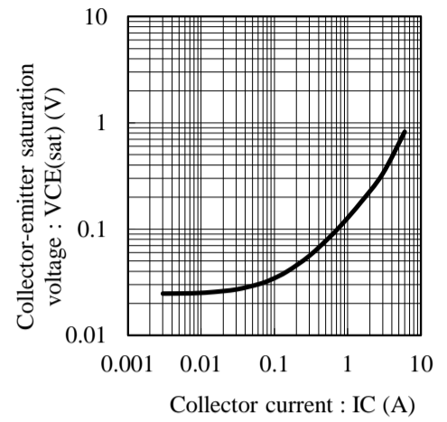
Fig.3 VCE(sat) - IC at IC/IB= 150, Ta= 25C
