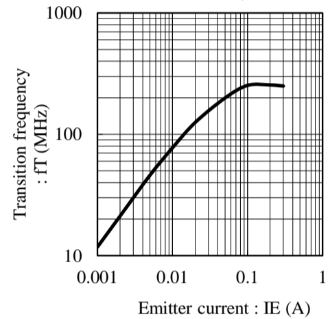
Fig.6 fT - IE at VCE= -2V, Ta= 25C
