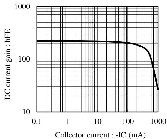
Fig.2 hFE - IC at VCE= -10V, Ta= 25C
