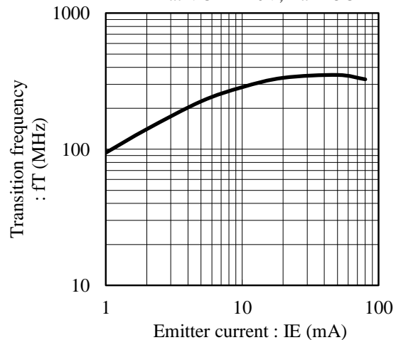
Fig.5 fT - IE at VCE= -20V, Ta= 25C
