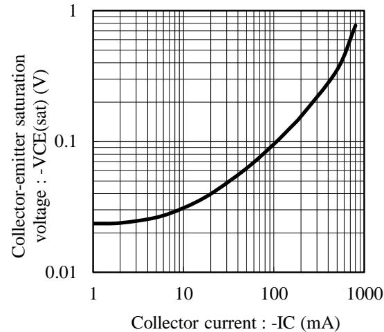
Fig.3 VCE(sat) - IC at IC/IB= 10, Ta= 25C
